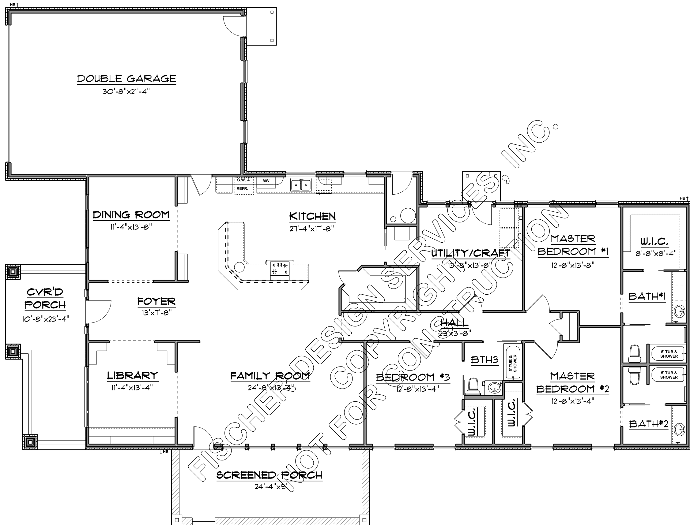
FLOORPLAN
