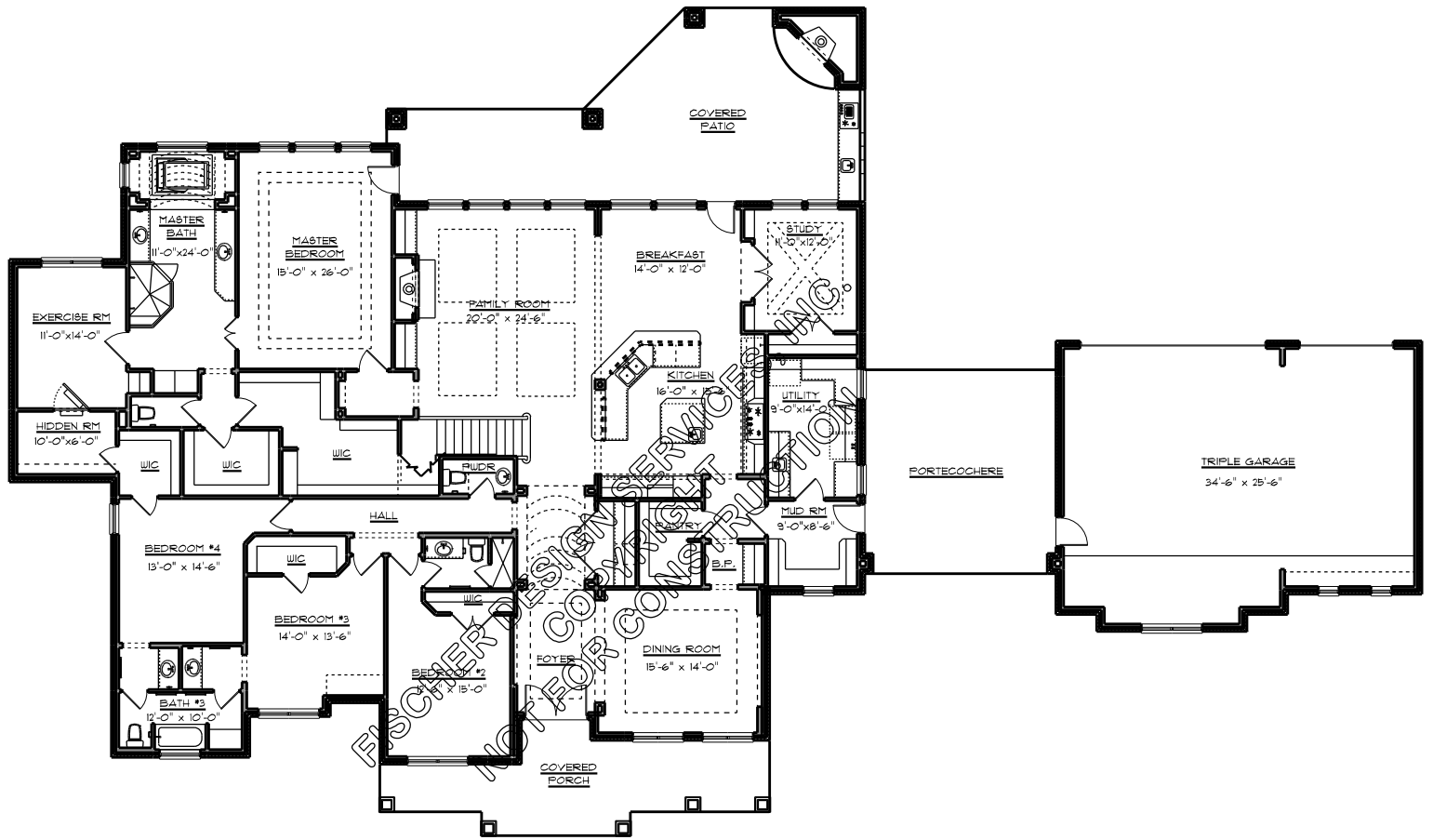
LOWER LEVEL FLOORPLAN
