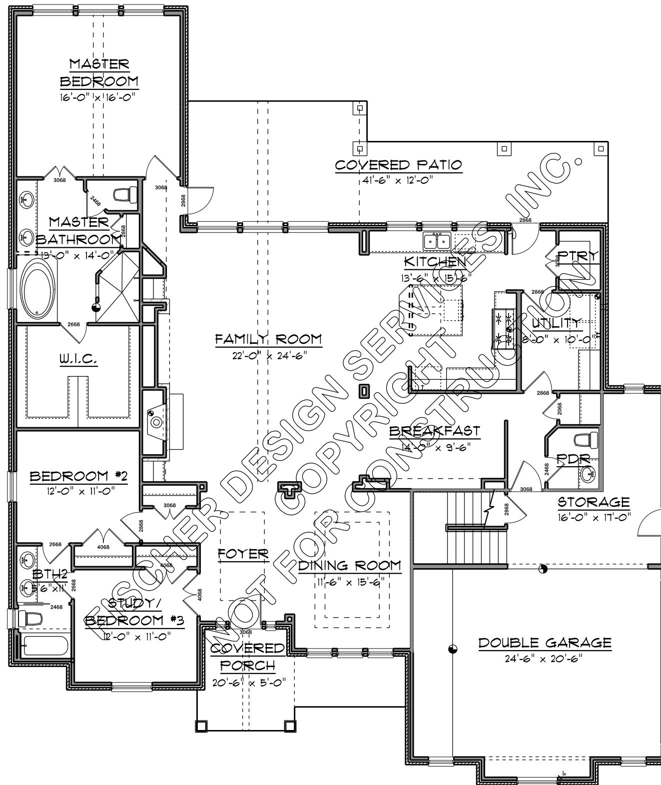
FRONT ELEVATION
