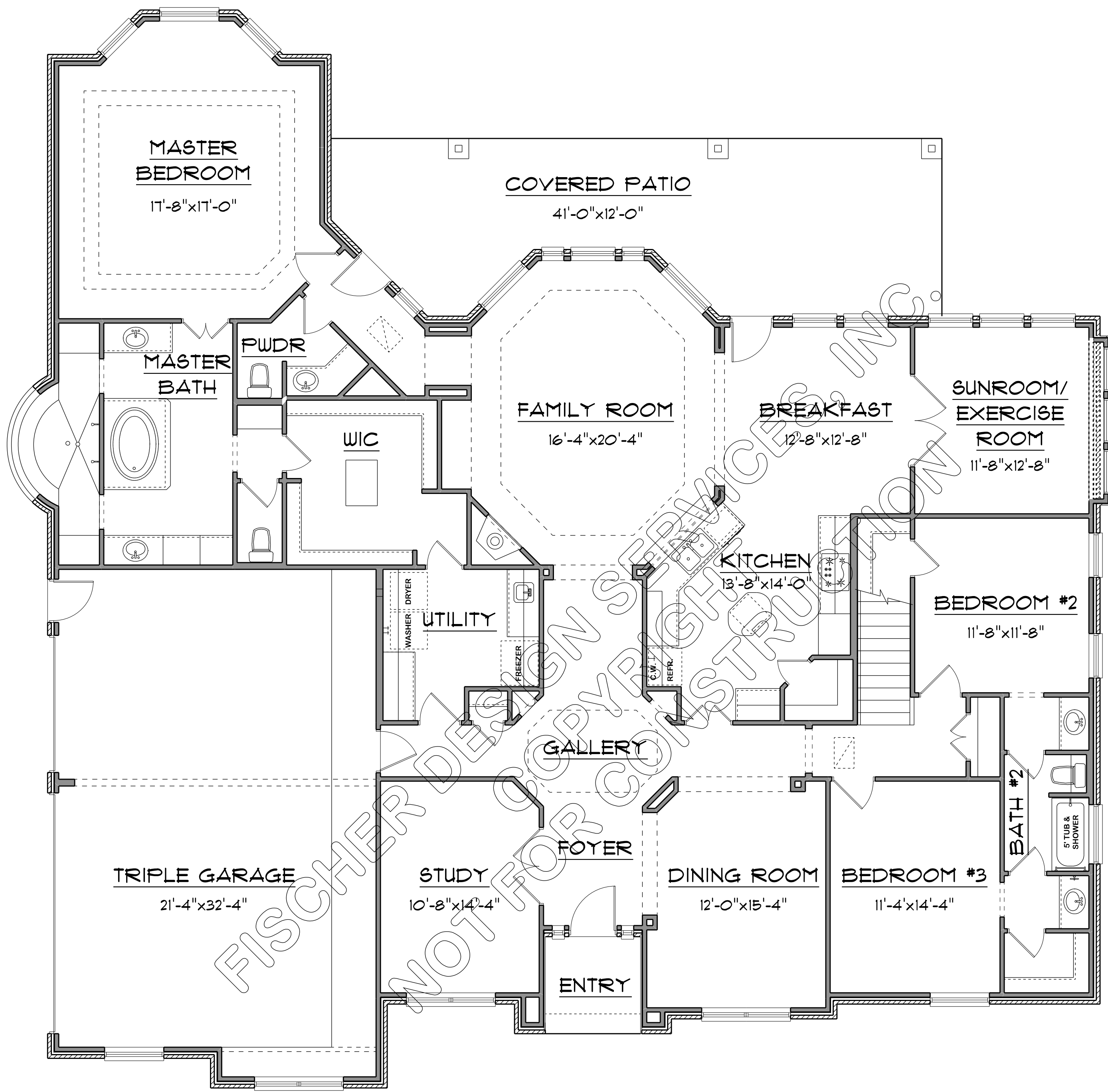
LOWER LEVEL FLOORPLAN
