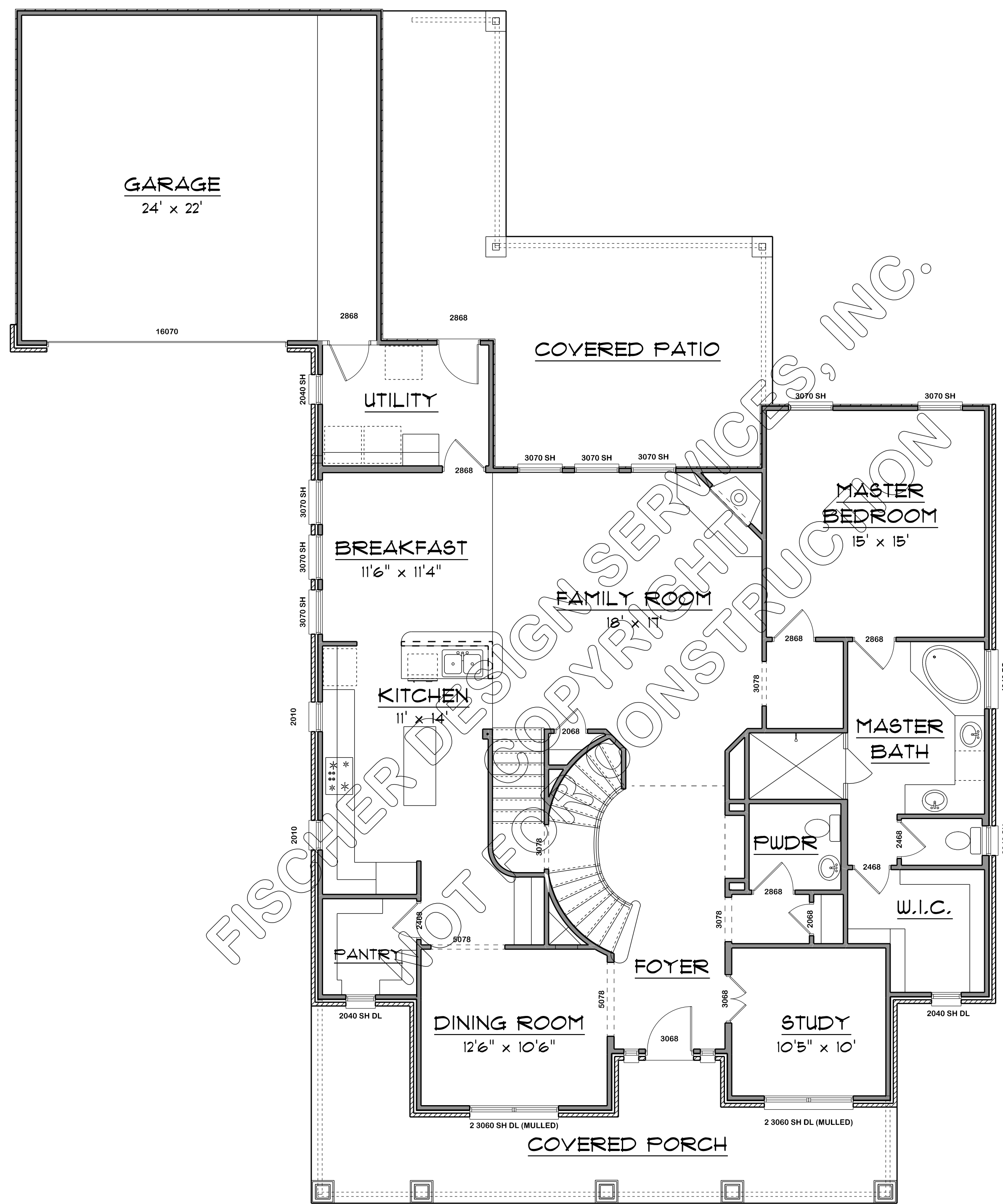
LOWER LEVEL FLOORPLAN
